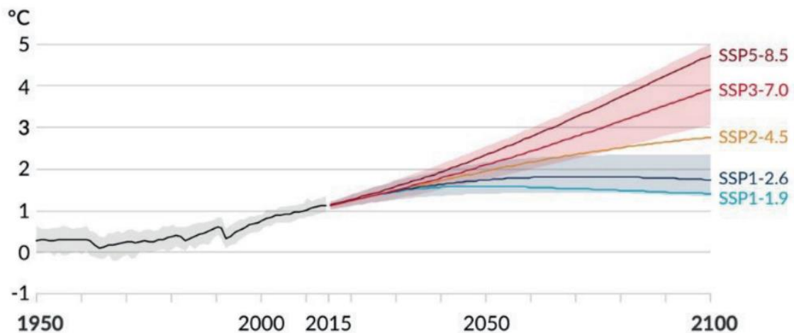
Fig 5: Different climatic scenarios and global temperature increases based on the IPCC. SSP5-8.5 is the highest warming pathway, SSP3-7.0 the second highest and so on. taken from Safeguarding chemical businesses in a changing climate How to prepare a Climate Change Adaptation Plan 2nd edition Note: SSP is shared socio-economic pathway
